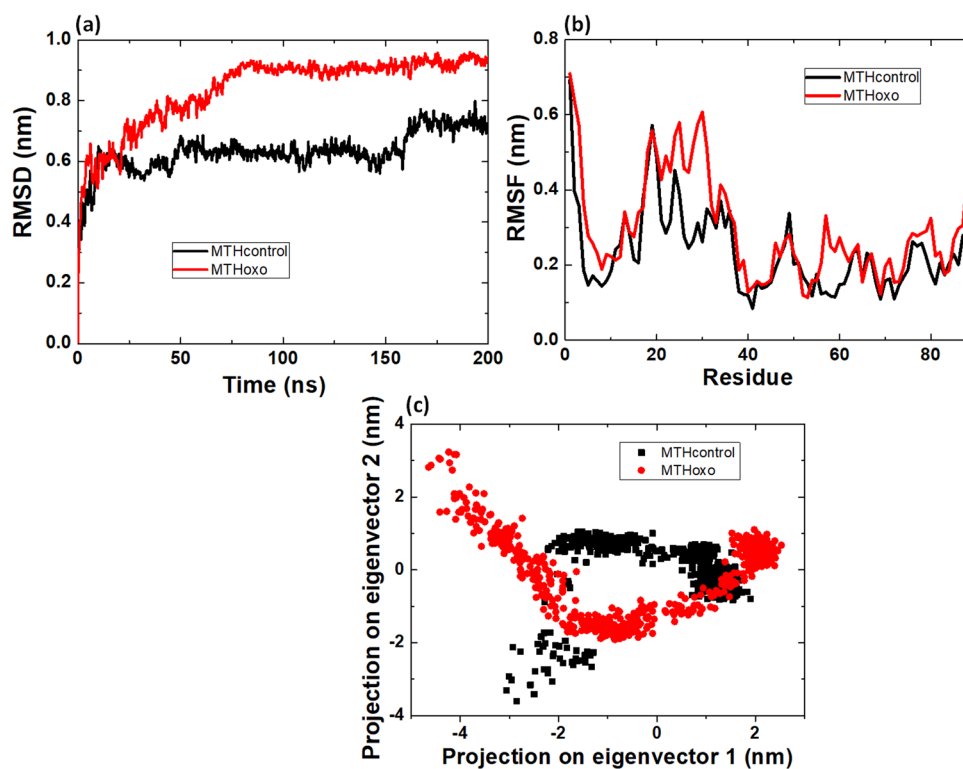
Figure 5. (a) RMSD, (b) RMSF and (c) projection of the motion in phase space along the first two principal eigenvectors values, of MTH control and MTHoxo.
