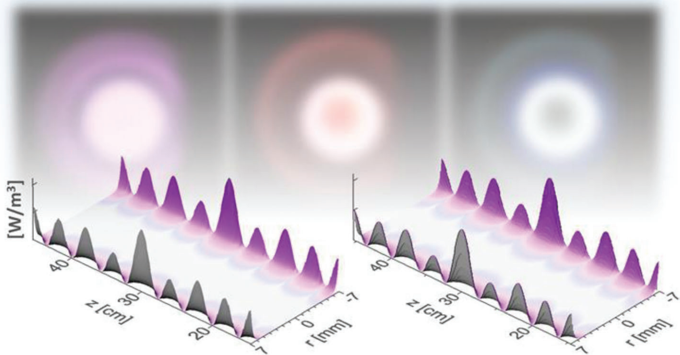
Quasi-neutral model
