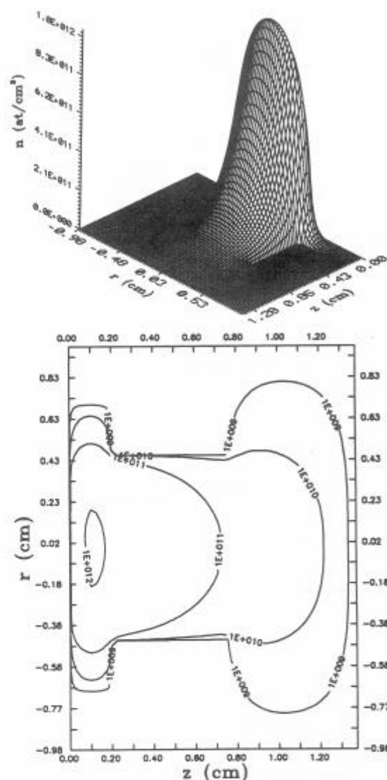
Figure 3. (a, Top) Density map for the sputtered neutral Mo atoms in a Mo/Ar glow discharge system ( p = 75 Pa, I = 3.53 mA/cm 2 , V = 881 V). (b, Bottom) Topographic representation of the concentration distribution of sputtered Mo atoms in a Mo/Ar GD system ( p = 75 Pa, I = 3.53 mA/cm 2 , V = 881 V, cross section of part a through the r,z plane).
