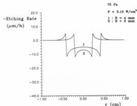
Figure 9. Theoretical crater profiles in a Mo sample after 1-h exposure to a GD-plasma: (1) standard cell configuration; (2) partial shielding of the sample. Discharge conditions: p = 75 \text{ Pa} , I = 3.53 \text{ mA/cm}^2 , V = 881 \text{ V} .
