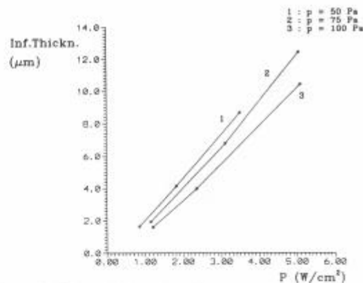
Figure 6. Calculated information thickness as a function of power density for three different pressures (Mo/Ar system).
