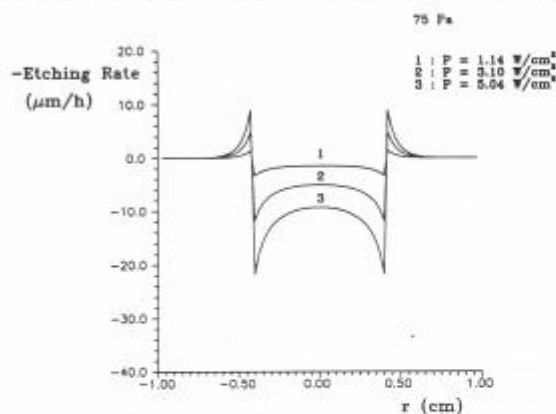
Figure 5. Theoretical crater profiles in a Mo sample after 1-h exposure to an Ar GD-plasma for three different power densities.
