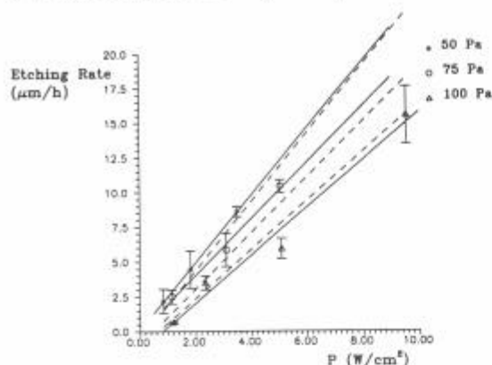
Figure 8. Measured and theoretically calculated etching rates for the Mo/Ar GD system as a function of power density for three different pressures.
