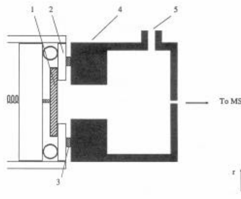
Figure 2. Standard GD cell: (1) sample (cathode); (2) mask; (3) insulator; (4) cell body (anode); (5) gas inlet.
