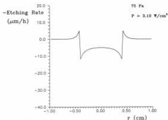
Figure 4. Theoretical crater profile in a Mo sample after 1-h exposure to an Ar GD-plasma ( p = 75 Pa, I = 3.53 mA/cm 2 , V = 881 V).
