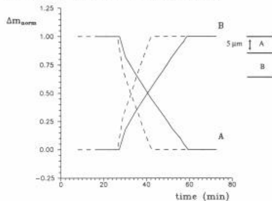
Figure 7. Theoretical depth profile for a layered sample (A, B). Solid lines, standard cell; dashed lines, partial shielding of the sample surface. Discharge conditions: p = 75 Pa, I = 3.53 mA/cm 2 , V = 881 V.
