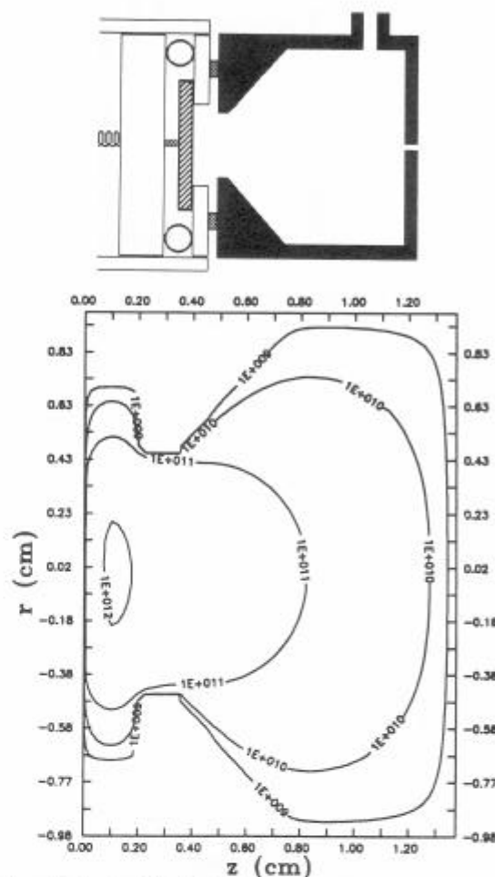
Figure 11. (a, Top) Modified cell configuration in which a part of the neck is cut off. (b, Bottom) Topographic representation of the concentration distribution of sputtered Mo atoms in a Mo/Ar GD system for the modified cell shown in part a ( p = 75 Pa, I = 3.53 \text{ mA/cm}^2 , V = 881 \text{ V} ).
