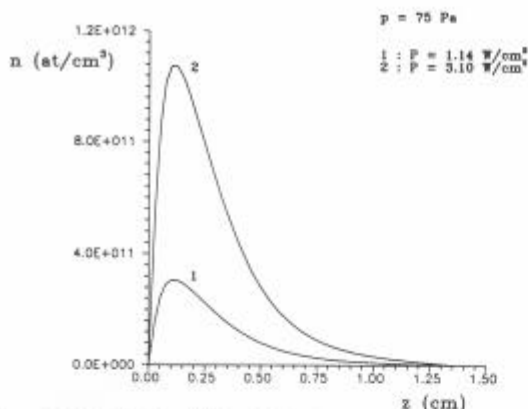
Figure 10. Calculated axial ( r = 0 ) density profile for Mo atoms in the standard GD cell for two different power densities ( p = 75 Pa).
