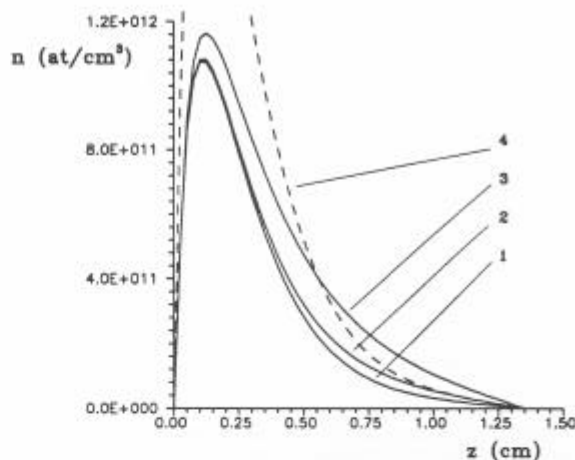
Figure 13. Calculated axial ( r = 0 ) density profiles for Mo atoms in the three cells investigated: (1) standard cell; (2) cell depicted in Figure 11a; (3) cell depicted in Figure 12a (discharge conditions for 1, 2, and 3: p = 75 Pa, I = 3.53 mA/cm 2 , V = 881 V); (4) standard cell with higher discharge power applied ( p = 75 Pa, I = 4.72 mA/cm 2 , V = 1069 V).
