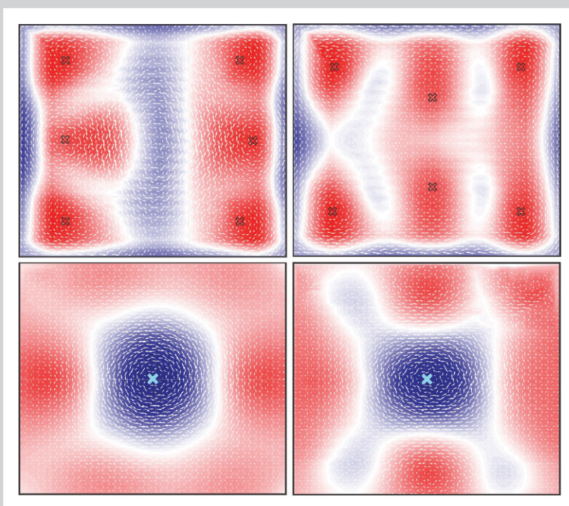
Fig.: Magnetic field induced vortices in graphene quantum dots
