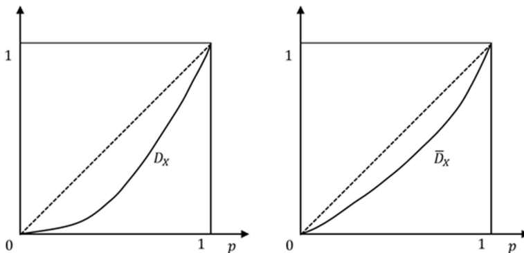
Figure 2: The downward diagonal dependence curve D_X (left) and upward diagonal dependence curve \bar{D}_X (right) of random vector X
