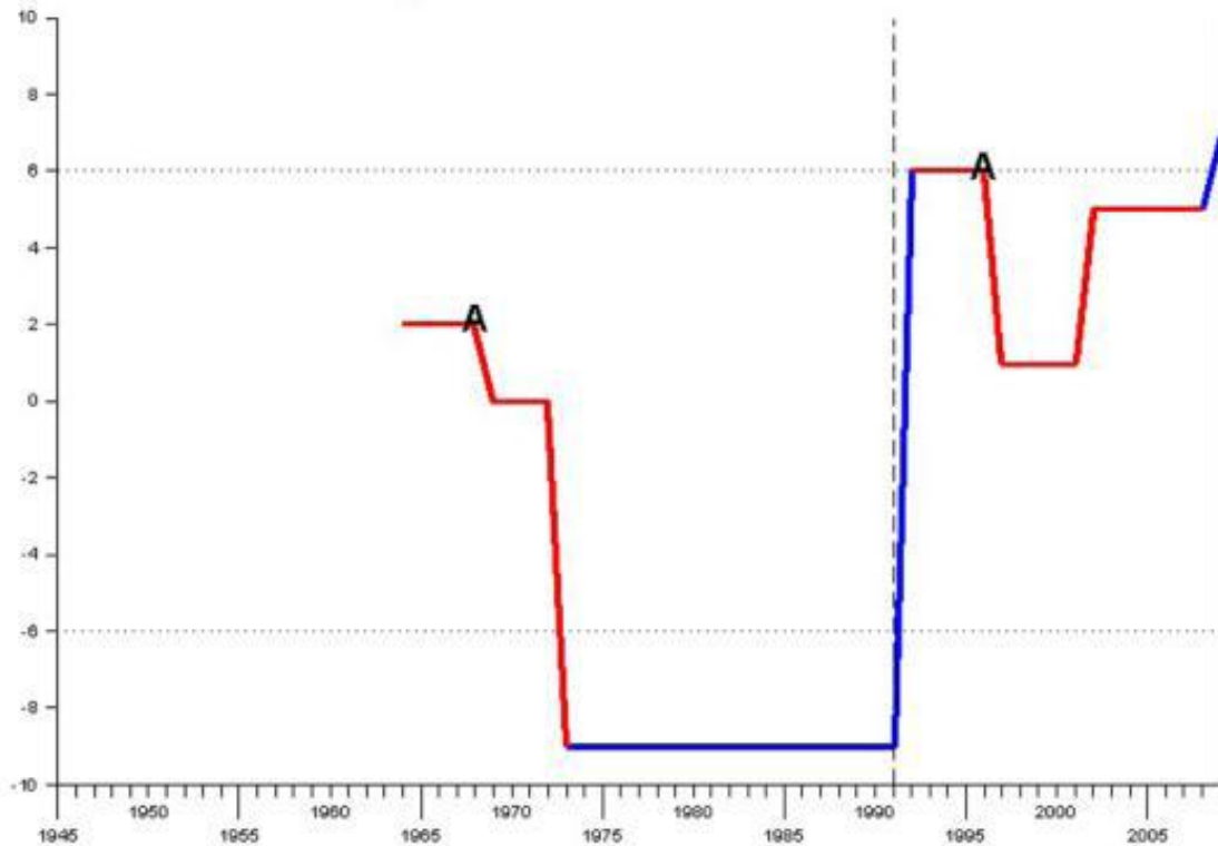
Figure 3. Source: Polity Dataset
