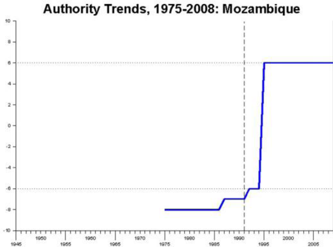
Figure 2. Source: Polity Dataset
