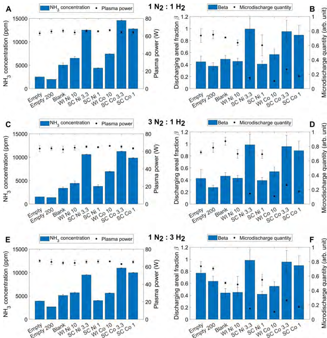
Figure 3-24: NH 3 outflow concentration and measured plasma power for a N 2 :H 2 ratio of 1:1 (A), 3:1 (C), and 1:3 (E). Discharging areal fraction \beta and microdischarge quantity for a N 2 :H 2 ratio of 1:1 (B), 3:1 (D), and 1:3 (F). The effect of the catalyst on the obtained NH 3 concentration can be dramatic, and a clear correlation with the discharge characteristics is apparent. In general, a lower microdischarge quantity and a higher discharging areal fraction are strongly beneficial for NH 3 synthesis.
