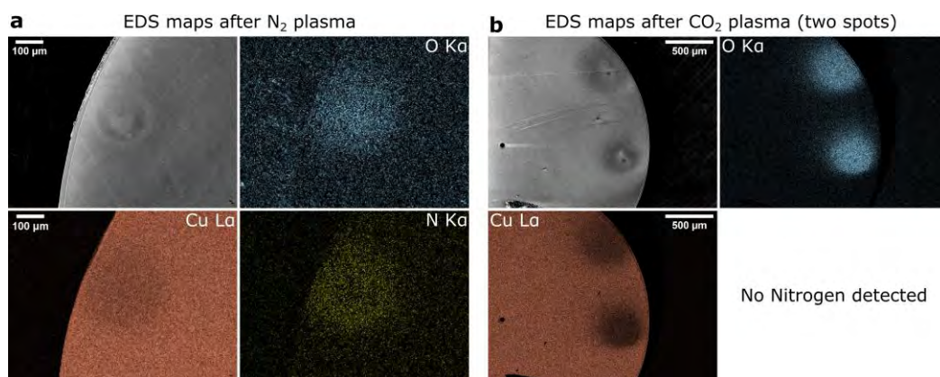
Figure 6-12: Comparison of N 2 and CO 2 plasma interactions on a Cu surface with reversed polarity (nozzle as a cathode). (a): EDS elemental maps reveal an O signal besides N after N 2 plasma treatment, probably caused by Cu oxide redeposition. (b): EDS elemental maps reveal the oxidized spots diameters of ca. 400 μm on the Cu foil for CO 2 plasma.
