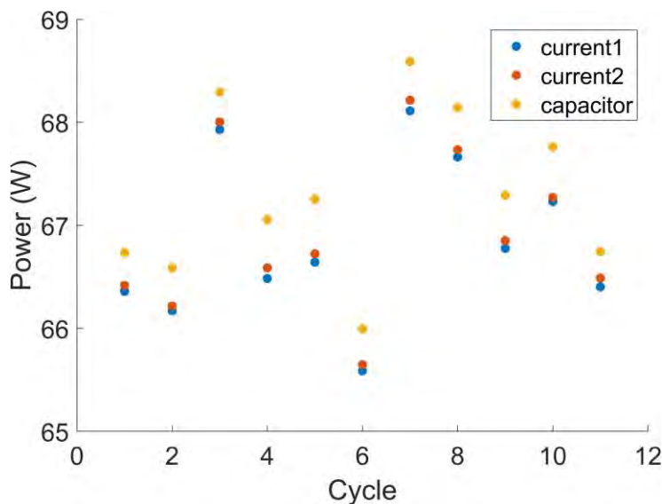
Figure A-1: Dissipated power per cycle in one snapshot, calculated using different methods. The cycle-to-cycle variation (due to inherent variation of the plasma discharge) is much larger than the deviation between different calculation techniques. The capacitor technique always yields a slightly higher power than the other techniques, which could be due to a small inaccuracy of the capacitance.
