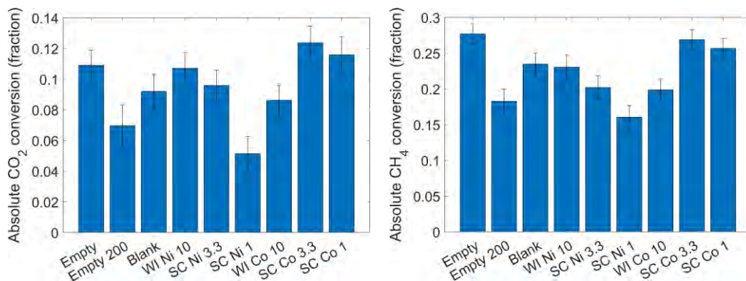
Figure A-21: Absolute CO 2 conversion (left) and CH 4 conversion (right) for DRM with a CO 2 /CH 4 ratio of 2:1. The catalysts do not increase (and in some cases notably decrease) the conversion compared to the empty reactor.
