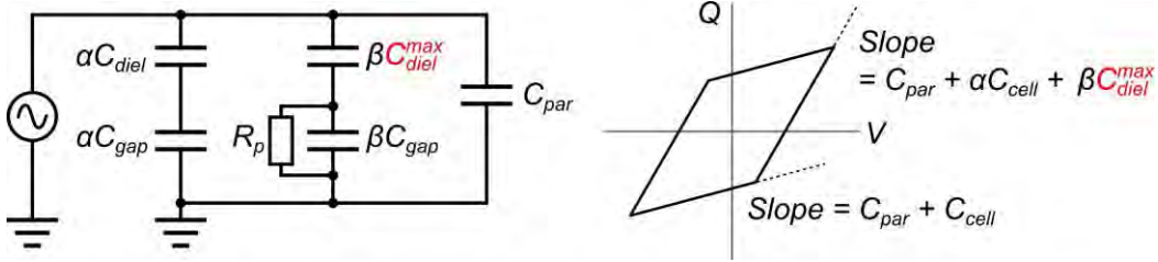
Figure 5-9: Proposed update to the equivalent circuit (left), and the corresponding interpretation of the capacitances in the voltage-charge diagram (right). Instead of using the theoretical dielectric capacitance that is based on the geometry of the reactor, the maximum measured dielectric capacitance is used in the equivalent circuit.
