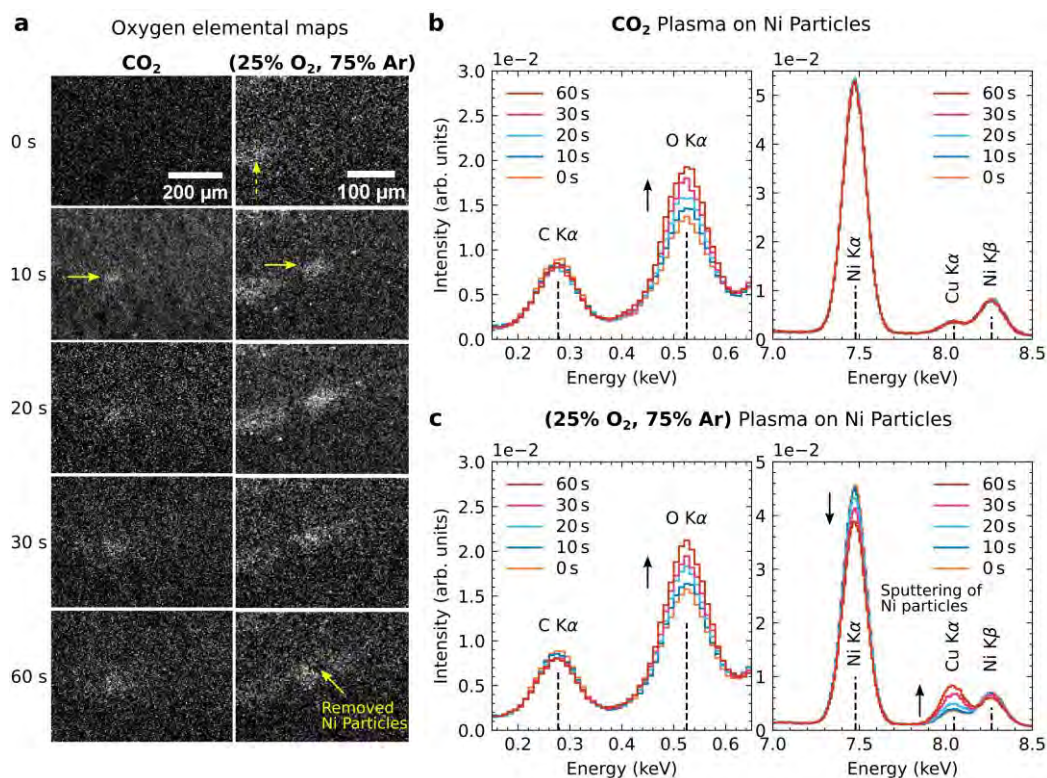
Figure 6-9: Local oxidation of Ni particles under CO 2 and O 2 /Ar plasma treatment. (a): Elemental maps showing the O Kα intensity for increasing plasma duration between 0 s to 60 s (top to bottom) for CO 2 plasma (left column) and O 2 /Ar plasma (right column) for similar discharge current (ca. 5 μA) and gap distance (ca. 250 μm). A spot of local oxidation is visible after 10 s (marked with horizontal arrows). The O-rich spot at 0 s for O 2 /Ar is from a previous experiment (dashed vertical arrow). (b, c): Comparison of extracted EDX signals in selected energy region for the O (left), and Ni and Cu energy regions (right). The increase in O signal for increasing plasma duration is visible. (c): For O 2 /Ar plasma, sputtering of Ni particles and subsequent exposition of the underlying Cu support reduces the Ni Kα signal and increases the Cu Kα signal. This effect is absent in (b), indicating a significantly reduced sputter yield for CO 2 plasma. For comparison, the EDX spectra in (b, c) were normalized to the integrated signals in the energy intervals [2 keV, 5 keV] and [10 keV, 14 keV] containing only bremsstrahlung background signal.
