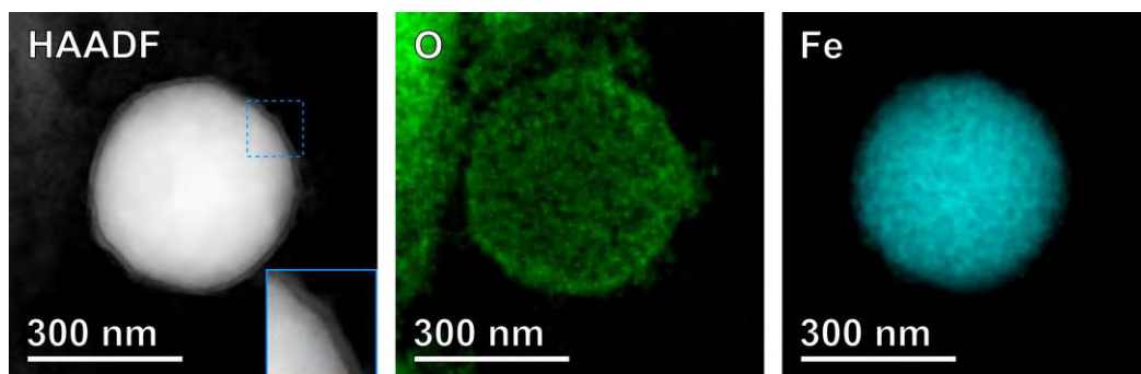
Figure 4-7: STEM-EDX characterization of a spherical steel particle generated in a \text{CO}_2 plasma. The HAADF-STEM image illustrates that the particle is covered by a lighter shell. The inset in the HAADF figure shows the indicated area at double the magnification. The oxygen EDX-map shows that the shell contains a clear oxygen signal, indicating that the shell is an oxide layer of the steel particle. The Fe map confirms that the particle contains Fe. The EDX characterization also yielded Ni and Cr signals (not shown), indicating that the particle is stainless steel.
