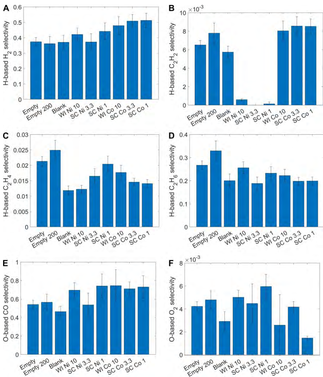
Figure 3-23: Selectivities based on DRM experiments with a \text{CO}_2/\text{CH}_4 ratio of 1:1. (A): H-based \text{H}_2 selectivity. (B): H-based \text{C}_2\text{H}_2 selectivity. (C): H-based \text{C}_2\text{H}_4 selectivity. (D): H-based \text{C}_2\text{H}_6 selectivity. (E): O-based CO selectivity. (F): O-based \text{O}_2 selectivity. The Co-based catalysts appear to yield higher selectivities toward \text{H}_2 and \text{C}_2\text{H}_2 and lower selectivities toward \text{C}_2\text{H}_4 , though these differences tend to be small.
