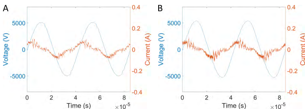
Figure 3-10: Voltage and discharge current oscillograms for \text{NH}_3 synthesis (1:1 ratio) with SC Ni 3.3 wt% (A) and SC Co 3.3 wt% (B). The corresponding microdischarge quantities are 0.1479 \pm 0.0062 (SC Ni 3.3 wt%, A) and 0.2661 \pm 0.0044 (SC Co 3.3 wt%, B). The more subtle differences in the microdischarge behavior are captured well by the microdischarge quantity.
