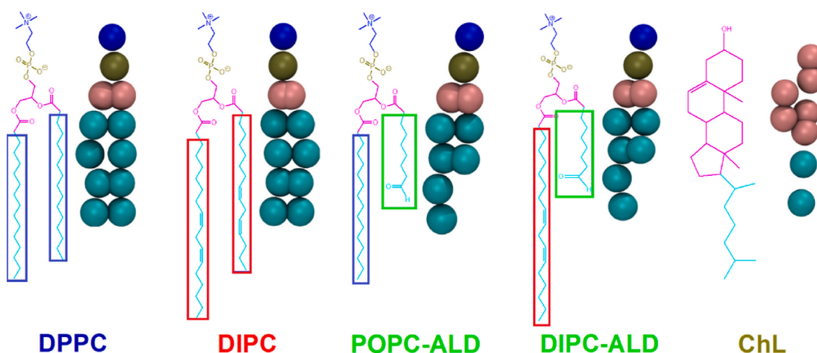
Fig. 1. Molecular structures of the lipids (DPPC, DIPC, POPC-ALD, DIPC-ALD) and cholesterol (ChL) molecules, and mapping of four heavy (non-hydrogen) atoms into one bead, for use in our CG MD simulations. Blue, dark yellow, pink and cyan colors represent the choline, phosphate, glycerol groups and acyl chains, respectively. The rectangles in red, blue and green represent unsaturated (chain A), saturated (chain B) and oxidized chains of the lipids, respectively. (For interpretation of the references to color in this figure legend, the reader is referred to the Web version of this article.)
