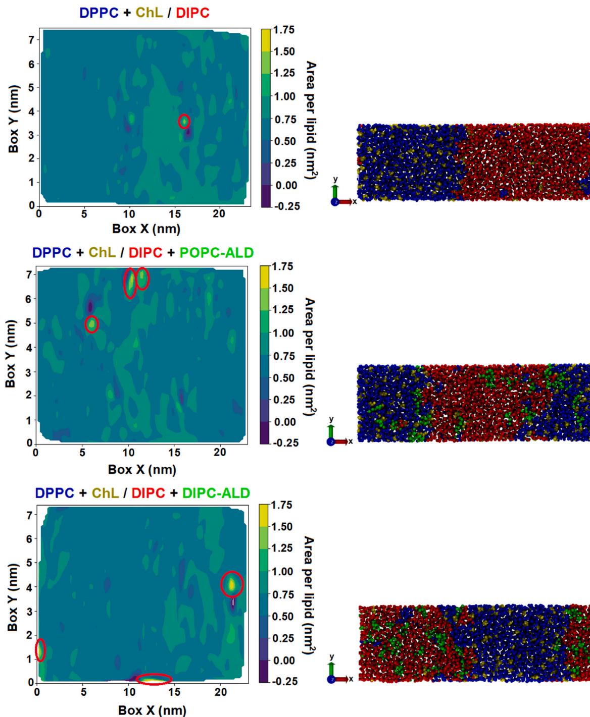
Fig. 4. Two-dimensional distribution of the area per lipid calculated at 12 \mu s of simulation (top view of only a single MD frame) (left side). Red circles indicate the positions where the area per lipid is higher. The right side also represents a top view of the membrane, but in this case the lipids are explicit. The box sizes in x and y -axes are the same in the right and left sides, but they are represented in different scales. (For interpretation of the references to color in this figure legend, the reader is referred to the Web version of this article.)
