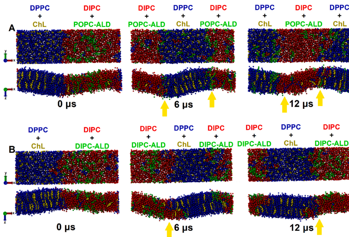
Fig. 2. Top view (upper panels) and side view (bottom panels) of the CG model membranes, where the Ld domain is composed either of (A) DIPC and POPC-ALD lipids or (B) DIPC and DIPC-ALD lipids. The Lo domain in both cases is composed of DPPC + ChL. Each bead is represented as a van der Waals sphere. Water molecules are not shown for the sake of clarity. The accumulation of POPC-ALD lipids at the interface after 6 and 12 \mu s of simulation in case (A) is indicated by the green van der Waals spheres, while in case (B) the DIPC-ALD lipids stay in the Ld domain, as also indicated by the green van der Waals spheres. Yellow arrows indicate the membrane constriction regions. (For interpretation of the references to color in this figure legend, the reader is referred to the Web version of this article.)
