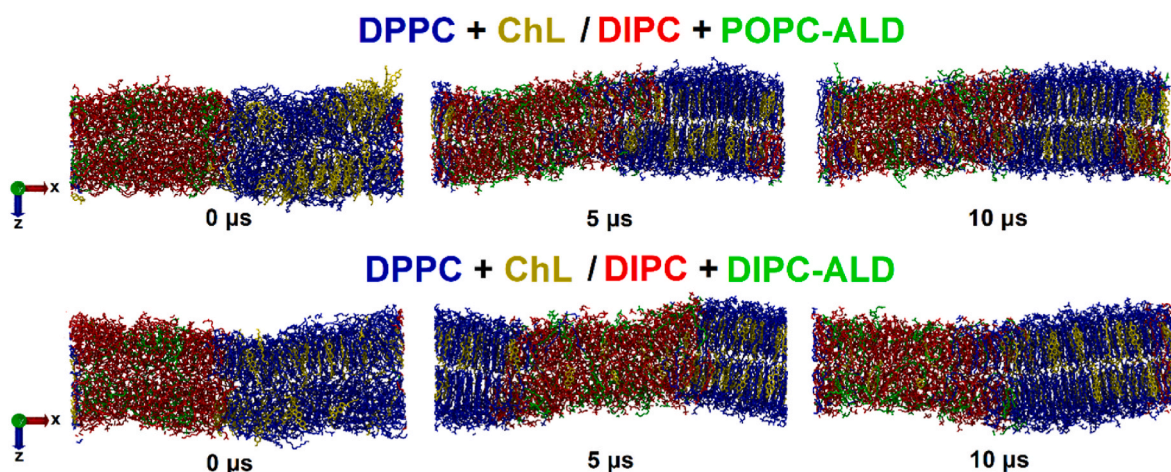
Fig. 5. Side view of the atomistic model membranes, where the Ld domain is composed either of DIPC and POPC-ALD lipids (upper panels) or DIPC and DIPC-ALD lipids (bottom panels). The Lo domain in both cases is composed of DPPC + ChL. Lipid molecules are represented as solid lines. Water molecules are not shown for the sake of clarity.
