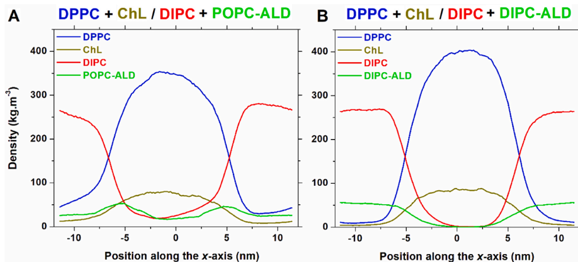
Fig. 3. Density profile of the CG model membranes, where the Ld domain is composed either of (A) DIPC and POPC-ALD lipids or (B) DIPC and DIPC-ALD lipids. The accumulation of POPC-ALD lipids at the Ld/Lo interface is clear from the maximum in the density profile (around -5 and +5 nm) (A), while no maximum at the interface is observed for the DIPC-ALD lipids (B). The values were calculated from the last 6 \mu s of simulations. The position x = 0 corresponds to the center of the Lo (DPPC + ChL) domain.
