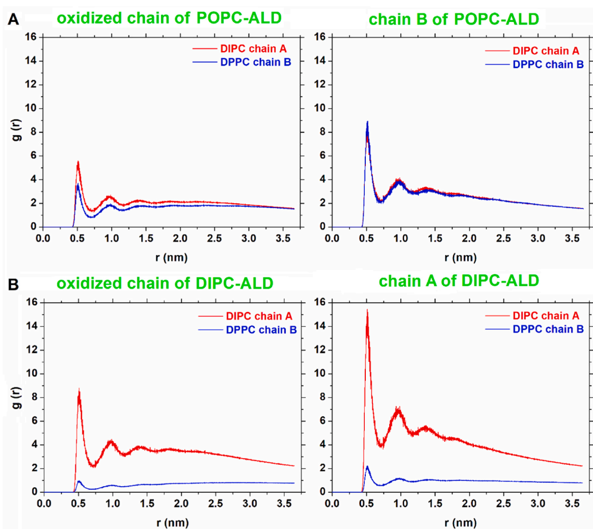
Fig. 6. Radial distribution function calculated for oxidized chains of POPC-ALD and DIPC-ALD from the last 6 \mu s of simulation. Chains A and B represent unsaturated and saturated chains, respectively. The values for chains A and B were calculated as an average between the two chains A or B of each lipid type.
