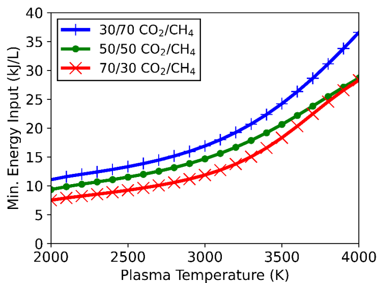
Figure S8. Minimum energy input required to achieve the final species distribution at the end of the plasma as a function of plasma temperature for the three different \text{CO}_2/\text{CH}_4 ratios (70/30, 50/50, 30/70).
