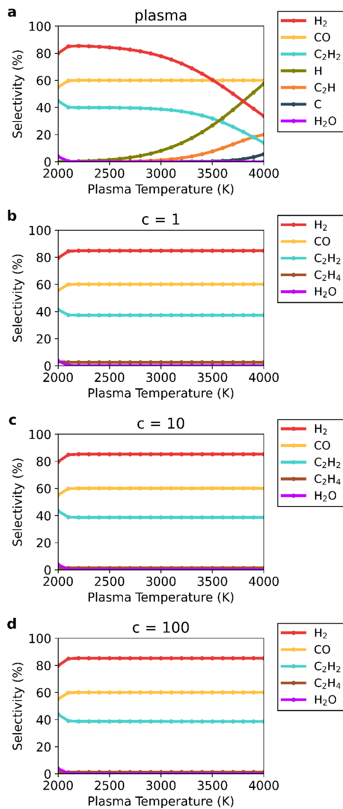
Figure S5. Selectivity of the main species (above 1%), as a function of the plasma temperature for the 30/70 \text{CO}_2/\text{CH}_4 ratio, at the end of the plasma (a), and at the end of the afterglow (b, c, d), for c -factors of 1 (b), 10 (c) and 100 (d). The \text{H}_2\text{O} and \text{C}_2\text{H}_4 selectivity curves overlap.
