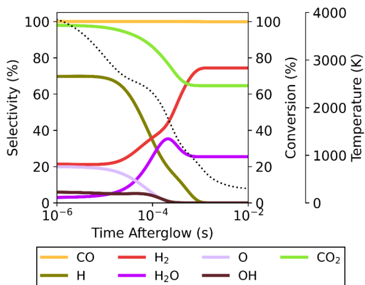
Figure S7. Time-evolution of the selectivity of the main species in the afterglow, starting from a plasma temperature of 4000 K for the 70/30 \text{CO}_2/\text{CH}_4 ratio and c-factor = 100. The evolution of the \text{CO}_2 conversion (lime green curve) and the gas temperature (dotted line) are also plotted, and shown on the right axis.
