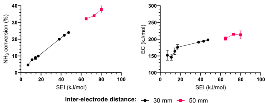
Fig. 7. NH 3 conversion (left) and EC (right) in the P2P arc plasma reactor, as a function of SEI per mole of NH 3 feed at two different inter-electrode distances. Feed flow rate – 20 Ln/min.
