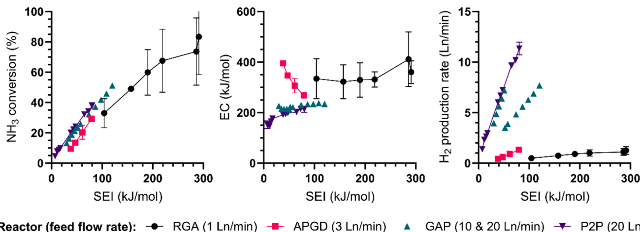
Fig. 8. NH 3 conversion (left), EC (middle), and H 2 production rate (right) in the investigated plasma reactors, as a function of SEI per mole of NH 3 feed. Each reactor is represented at its best-performing feed flow rate: 1 Ln/min for RGA, 3 Ln/min for APGD, 10 and 20 Ln/min for GAP, and 20 Ln/min for P2P. Data for the GAP is plotted for both 10 and 20 Ln/min to compare its performance over a wider SEI range.
