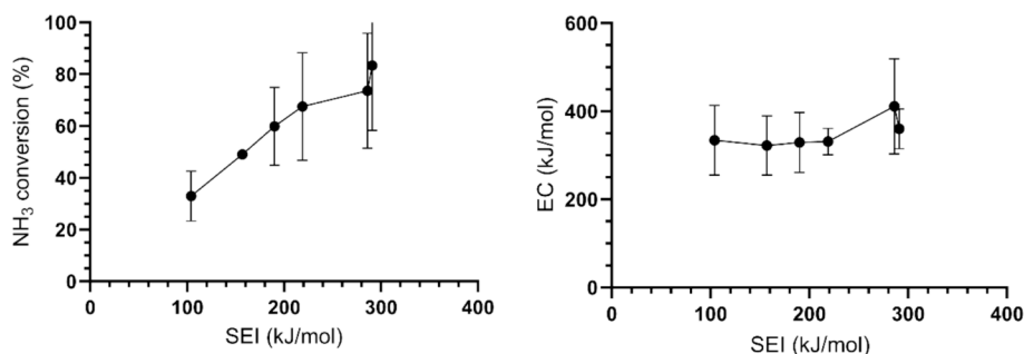
Fig. 3. \text{NH}_3 conversion (left) and EC (right) in the RGA plasma reactor, as a function of SEI per mole of \text{NH}_3 feed. Feed flow rate – 1 Ln/min.
