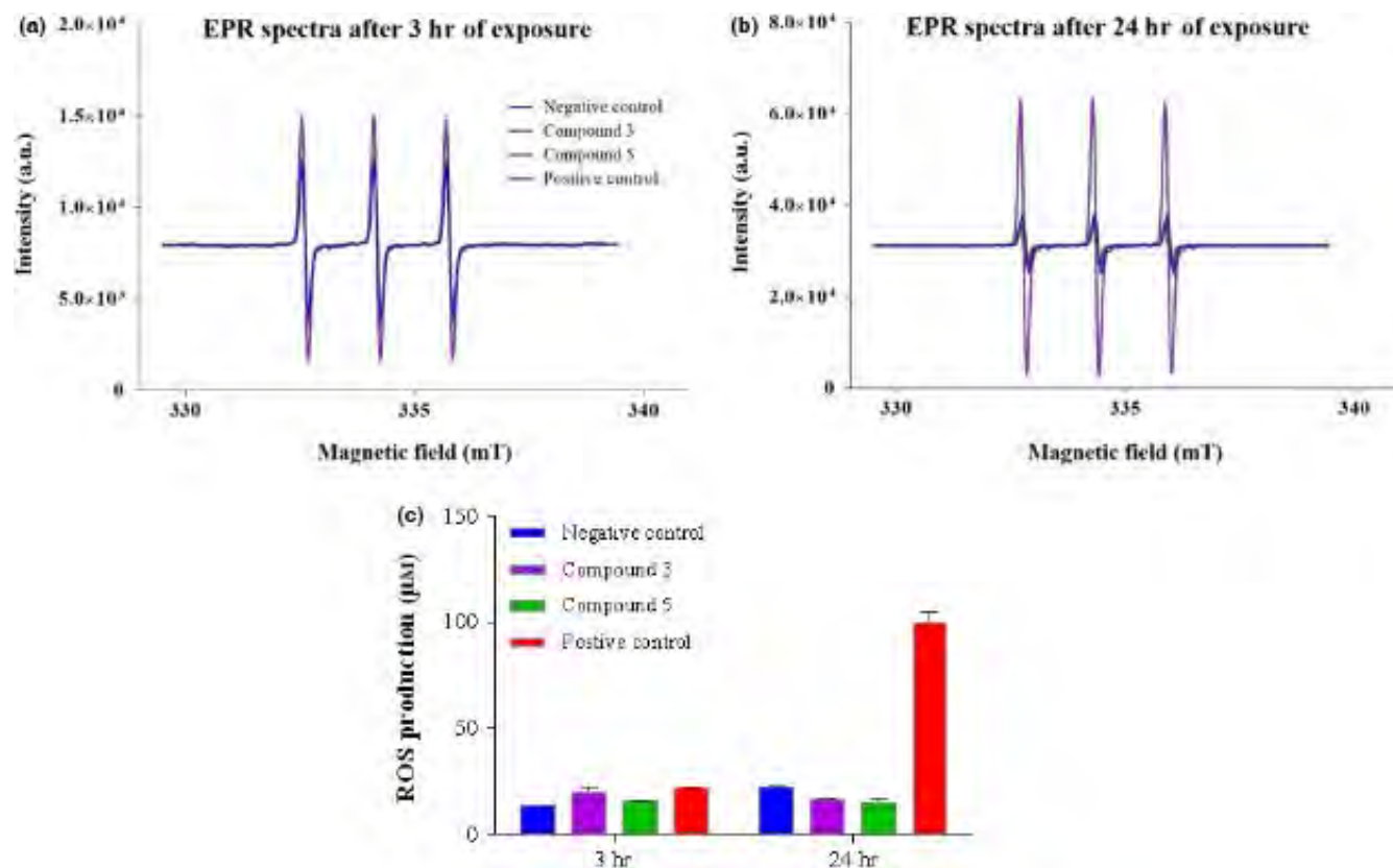
FIGURE 3 (a) EPR spectra measured after 3 hr and (b) 24 hr to compound 3 and compound 5 . Negative control includes the EPR spectra of unexposed cells, while the positive control contains the EPR spectra of cells exposed to phorbol myristate acetate (PMA). The signal intensity in function of ROS production is measured in arbitrary units. (c) The simulated spectra were double integrated ( \Delta n = 1.58 mT). The numbers presented are averages of two measurements [Colour figure can be viewed at wileyonlinelibrary.com ]
