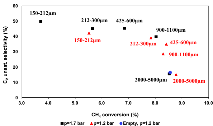
Fig. 7 Carbon selectivity to unsaturated C 2 species plotted against the conversion of CH 4
