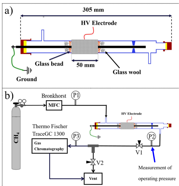
Fig. 1 a Schematic diagram of the applied packed bed DBD plasma reactor. The schematic drawing is color coded to distinguish the different materials: quartz glass reactor (blue), end plastic plugs (dark red), silicone O ring (yellow), stainless steel rod (black), stainless steel mesh (grey), glass beads (orange), insulated grounded wire (green), insulated HV cable (red). b Schematic representation of the experimental setup, showing the gas lines, position of manometers (P1–P3), needle valves (V1 and V2) and GC. The operating pressure in the reactor was measured using P2 located just after the reactor (Color figure online)
