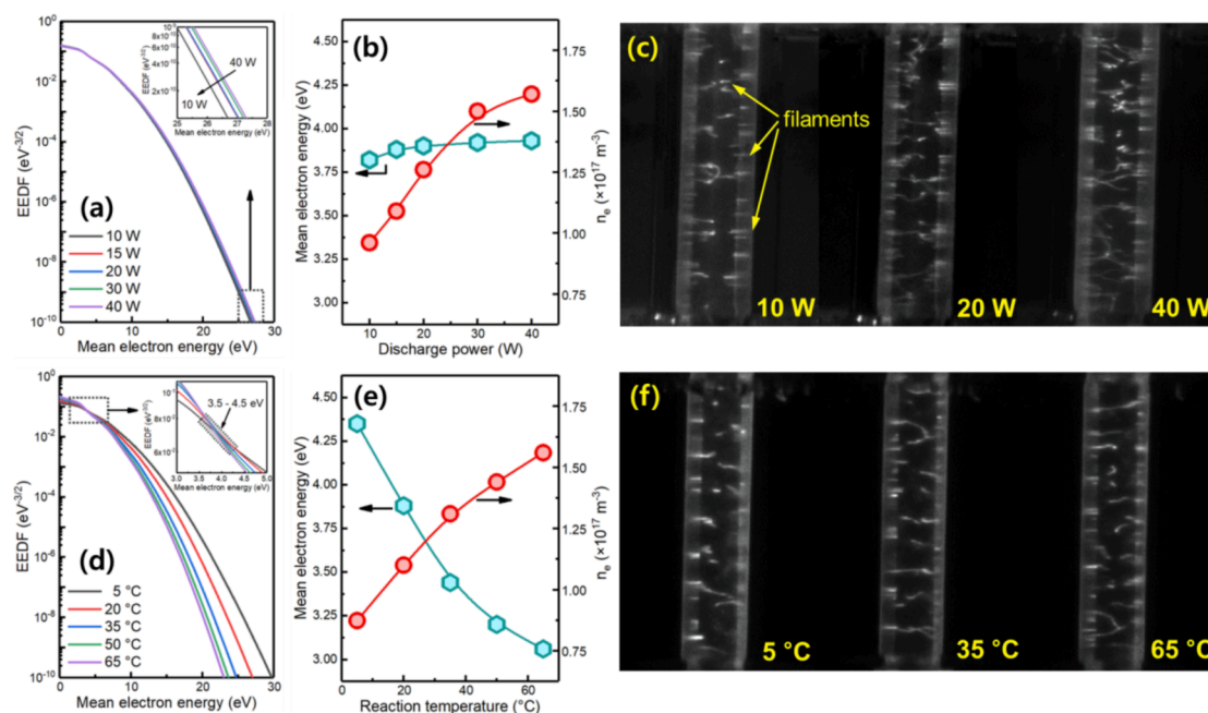
Fig. 6. Calculated electron energy distribution function (EEDF), mean electron energy and mean electron density, and ICCD images of the filamentary discharge (exposure time: 50 ms) at (a-c) different discharge powers (at a fixed temperature of 20 °C) and (d-f) different reaction temperatures (at a fixed discharge power of 15 W).
