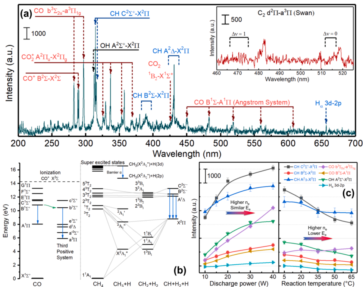
Fig. 8. (a) Typical optical emission spectra for the CO 2 -CH 4 plasma (discharge power: 40 W). (b) Electronic energy levels and terms for CO and CH 4 (including dissociation), as reproduced from literatures [53–55]. The blue arrows indicate the detected emissions; the green arrow denotes the collision-induced intersystem crossing. (c) Effect of discharge power and reaction temperature on the intensity of different emission lines, originating from various excited species in the CO 2 -CH 4 plasma derived from Figure S4 (CH(C 2 Σ + - X 2 Π) 314 nm; CH(B 2 Σ - X 2 Π) 387 nm; CH(A 2 Δ - X 2 Π) 431 nm; OH(A 2 Σ + - X 2 Π) 309 nm; CO(b 3 Σ 2u - a 3 Π 1g ) 283 nm; CO(B 1 Σ - A 1 Π) 451 nm; H α (3d - 2p) 656 nm). (For interpretation of the references to colour in this figure legend, the reader is referred to the web version of this article.)
