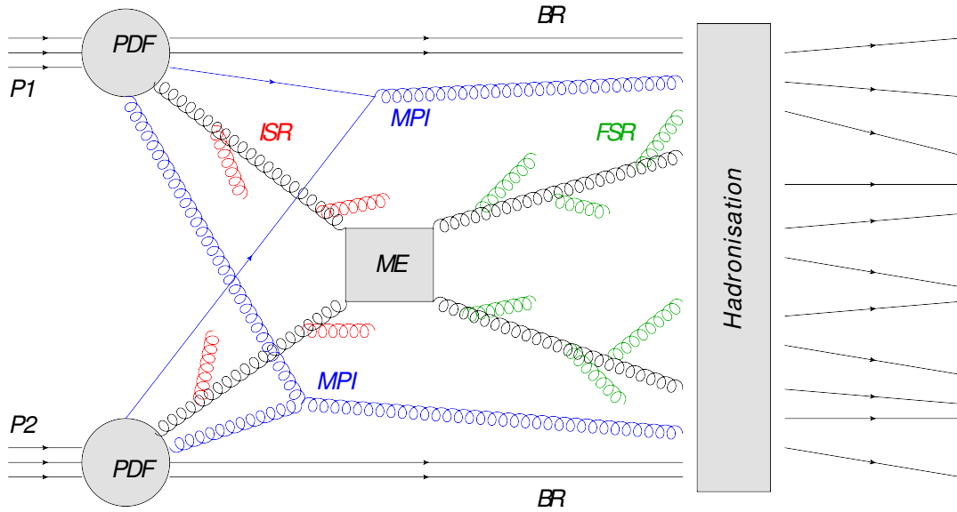
Figure 3.1.: Schematic view of a hadron-hadron collision with its different components indicated. It represents the evolution of an initial state (left) to the final state (right) with all its (non-)perturbative dynamics, which are explained in the text.
