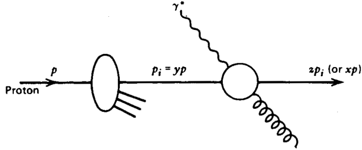
Figure 2.6.: Definition of the different momentum fractions after the inclusion of a \gamma^* q \rightarrow qq process. [12]
