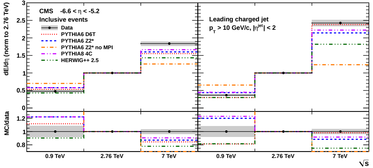
Figure 9.38.: Energy density in the pseudorapidity range -6.6 < \eta < -5.2 in inclusive events (left) and in events with a charged-particle jet in the range |\eta^{\text{jet}}| < 2 (right) as a function of \sqrt{s} , normalised to the energy density at \sqrt{s} = 2.76 TeV. The p_T threshold used for jets is 10 GeV/c at all centre-of-mass energies. Corrected results are compared to the PYTHIA and HERWIG++ MC models. Statistical uncertainties are smaller than the marker size, while the grey band represents the statistical and systematic uncertainties added in quadrature.
