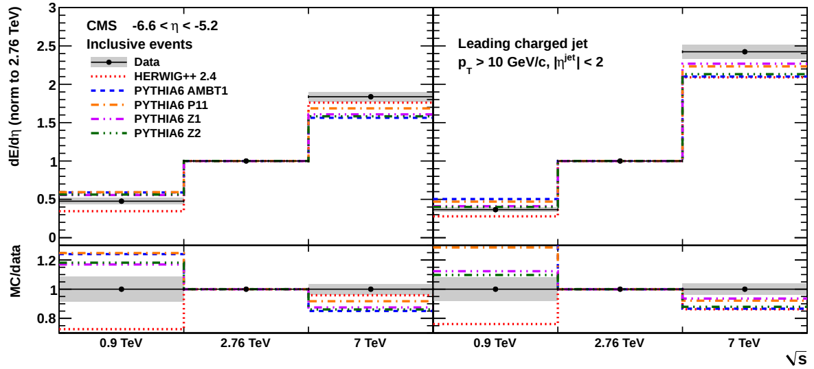
Figure 9.40.: Energy density in the pseudorapidity range -6.6 < \eta < -5.2 in inclusive events (left) and in events with a charged-particle jet in the range |\eta^{\text{jet}}| < 2 (right) as a function of \sqrt{s} , normalised to the energy density at \sqrt{s} = 2.76 TeV. The p_T threshold used for jets is 10 GeV/c at all centre-of-mass energies. Corrected results are compared to additional models of PYTHIA and an older version of HERWIG++. Statistical uncertainties are smaller than the marker size, while the grey band represents the statistical and systematic uncertainties added in quadrature.
