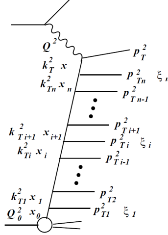
Figure 3.3.: Graphical presentation of a parton shower ladder diagram in a DIS process. The kinematics are explained in the text. [18]
