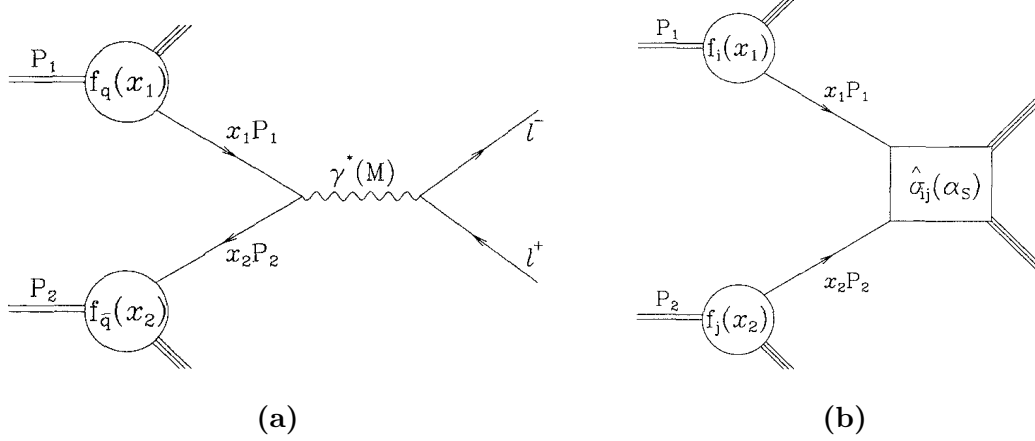
Figure 2.7.: (a) Lepton pair production in the Drell-Yan process through a hard scattering of two partons ( x_1 P_1 and x_2 P_2 ) from the incoming hadrons. (b) The parton model description for a general hard scattering process ( \hat{\sigma}_{ij}(\alpha_S) ) [11]
