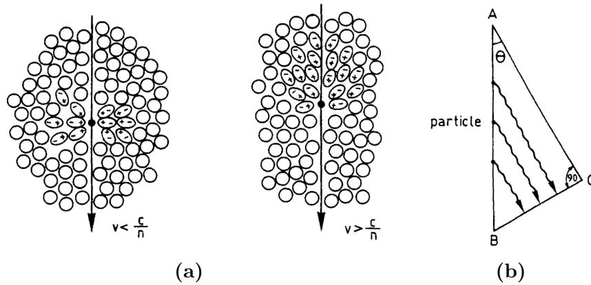
Figure 6.1.: (a) Dipole creation by the passage of relativistic charged particles in a dielectric medium. (b) Derivation of the Čerenkov angle. [85]
