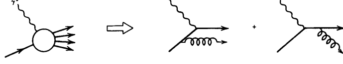
Figure 2.4.: \gamma^* q \rightarrow qqg contributions to the inclusive ep \rightarrow eX process. [12]
