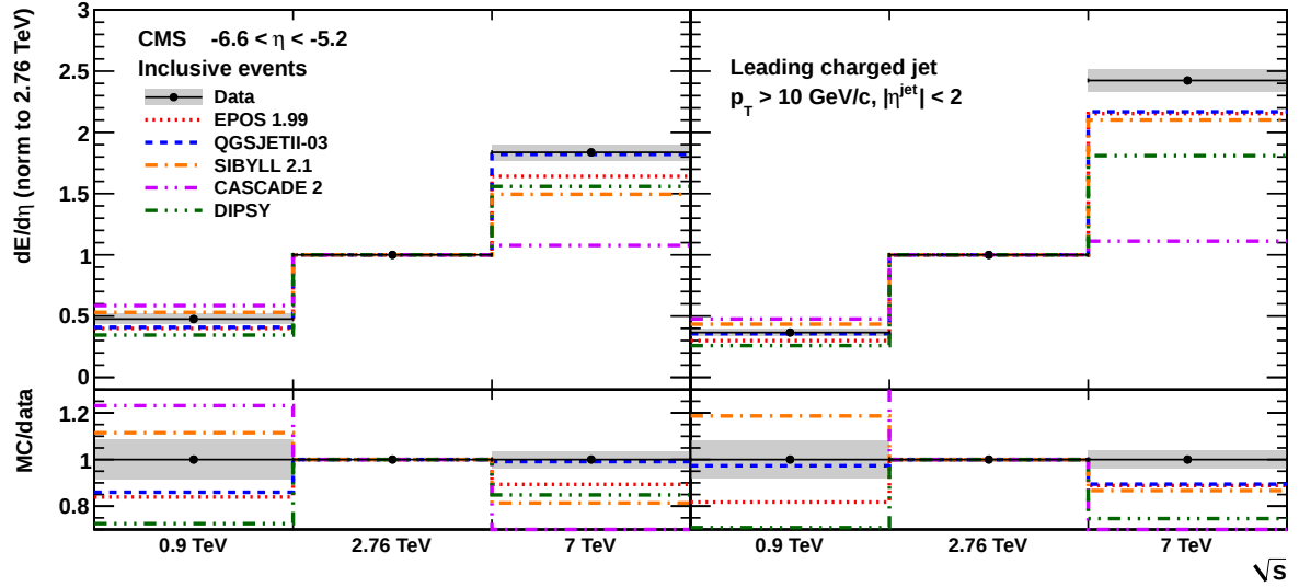
Figure 9.39.: Energy density in the pseudorapidity range -6.6 < \eta < -5.2 in inclusive events (left) and in events with a charged-particle jet in the range |\eta^{jet}| < 2 (right) as a function of \sqrt{s} , normalised to the energy density at \sqrt{s} = 2.76 TeV. The p_T threshold used for jets is 10 GeV/c at all centre-of-mass energies. Corrected results are compared to MC models used in cosmic ray physics and to CASCADE and DIPSY. Statistical uncertainties are smaller than the marker size, while the grey band represents the statistical and systematic uncertainties added in quadrature.
